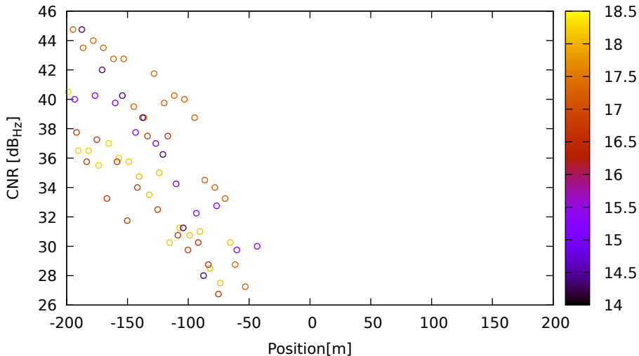
CNR vs position for G32 (L1) on LeicaGS18 - DOY 262 jam. 2
