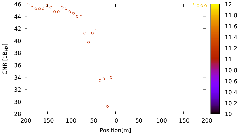
CNR vs position for G32 (L1) on LeicaGS18 - DOY 262 jam. 3
