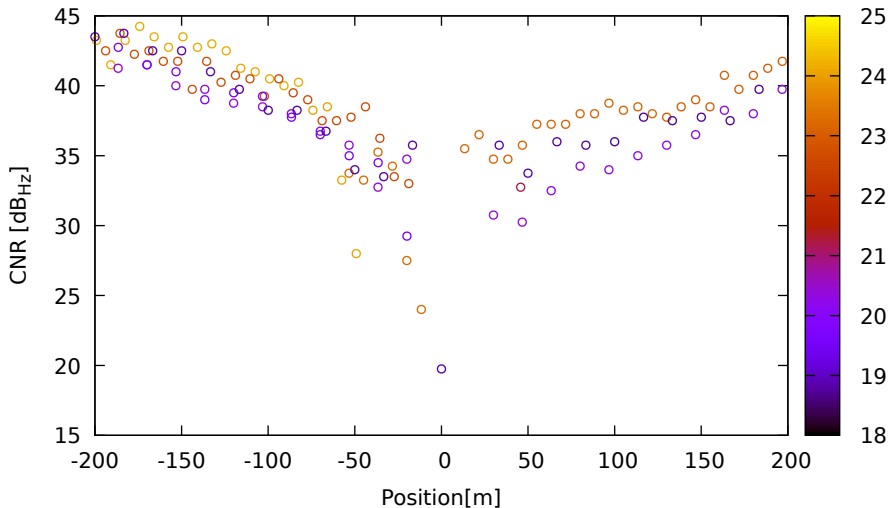
CNR vs position for G32 (L2) on LeicaGS18 - DOY 262 jam. 1
