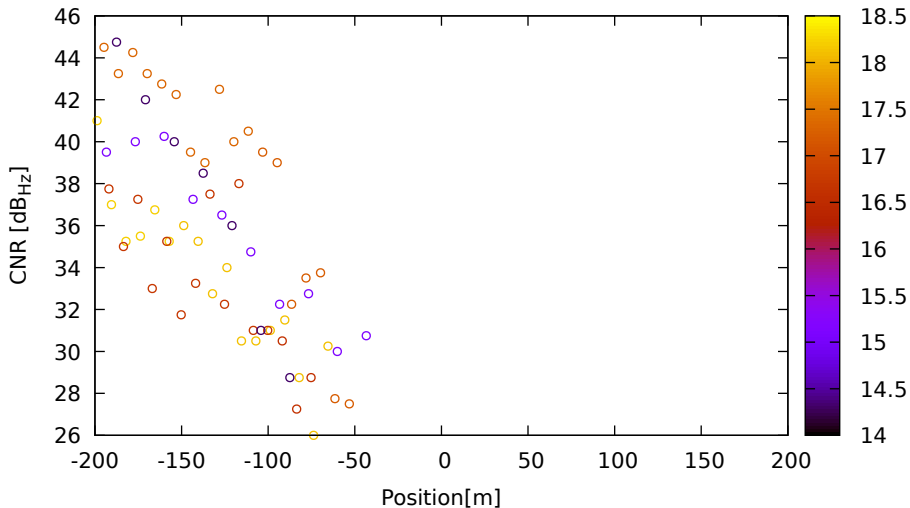
CNR vs position for G32 (L2) on LeicaGS18 - DOY 262 jam. 2
