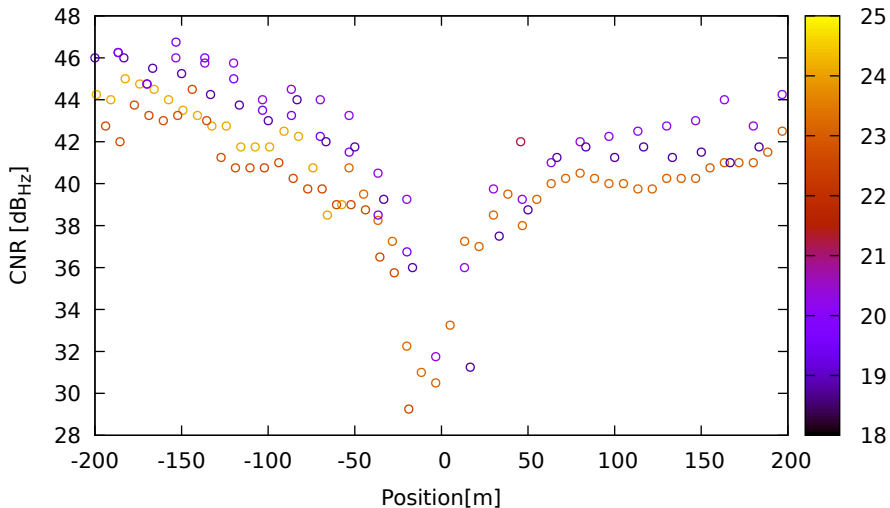
CNR vs position for G32 (L5) on LeicaGS18 - DOY 262 jam. 1
