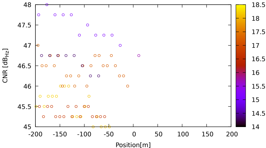
CNR vs position for G32 (L5) on LeicaGS18 - DOY 262 jam. 2
