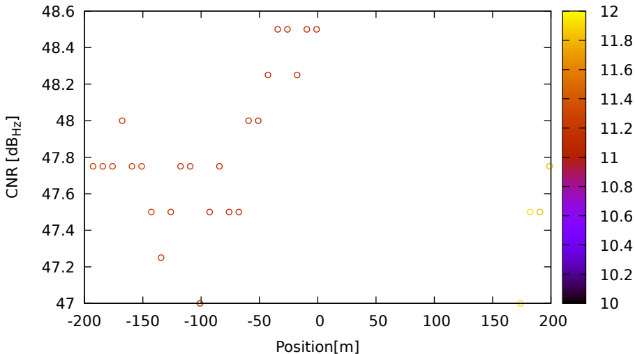
CNR vs position for G32 (L5) on LeicaGS18 - DOY 262 jam. 3
