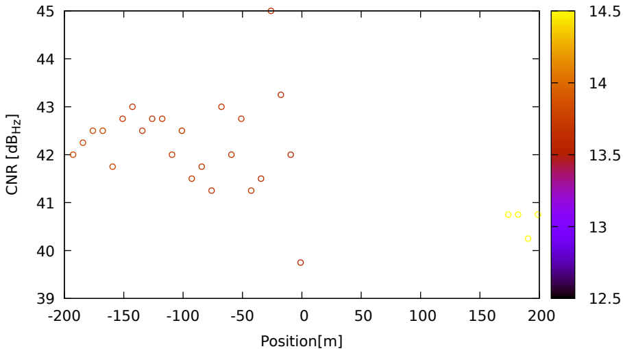
CNR vs position for R07 (G1) on LeicaGS18 - DOY 262 jam. 3
