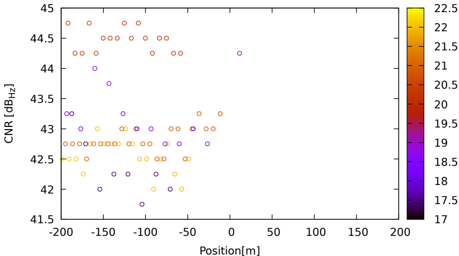
CNR vs position for R07 (G2) on LeicaGS18 - DOY 262 jam. 2
