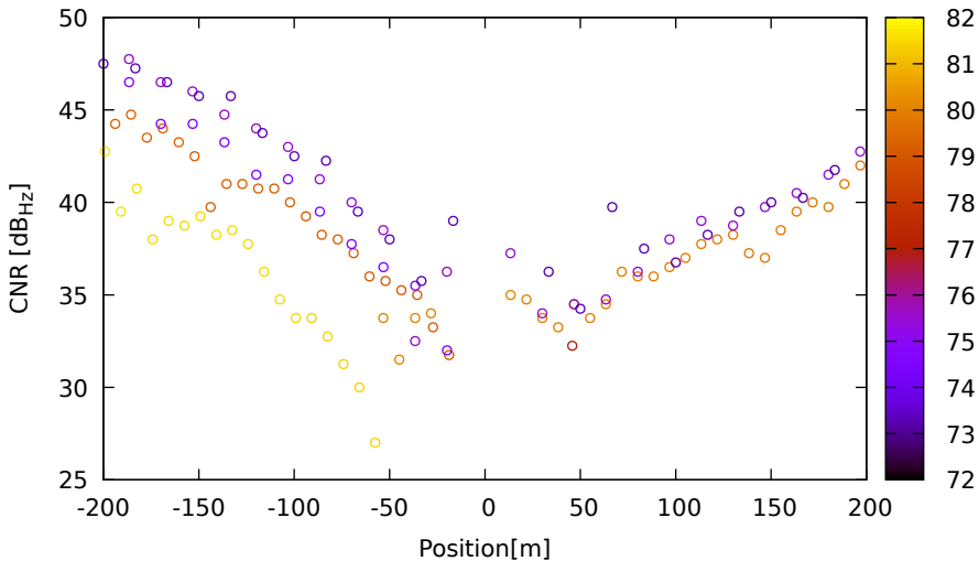
CNR vs position for R08 (G1) on LeicaGS18 - DOY 262 jam. 1
