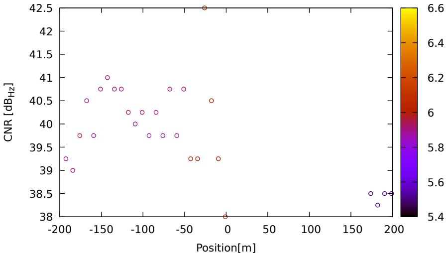
CNR vs position for R09 (G1) on LeicaGS18 - DOY 262 jam. 3
