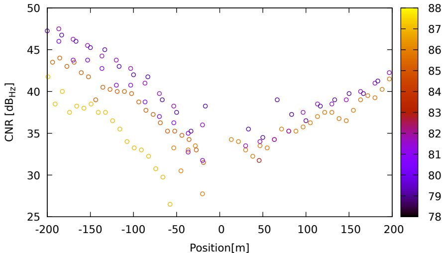
CNR vs position for R23 (G1) on LeicaGS18 - DOY 262 jam. 1
