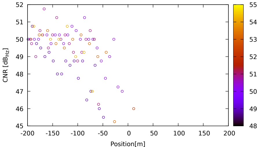
CNR vs position for R24 (G1) on LeicaGS18 - DOY 262 jam. 2
