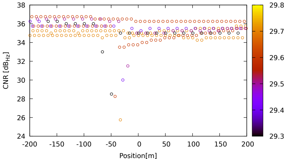
CNR vs position for C06 (B1) on Xiaomi11T - DOY 262 jam. 2
