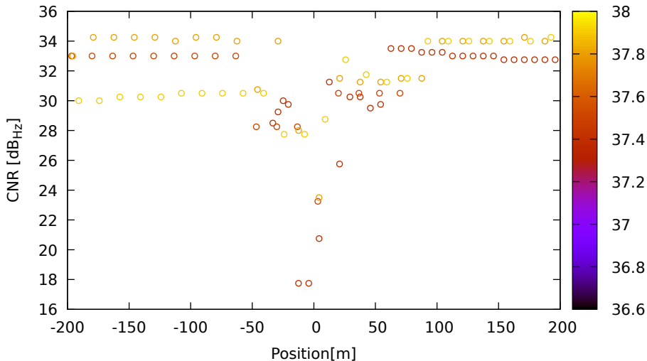
CNR vs position for C09 (B1) on Xiaomi11T - DOY 262 jam. 1
