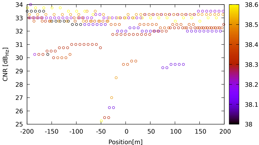
CNR vs position for C09 (B1) on Xiaomi11T - DOY 262 jam. 2
