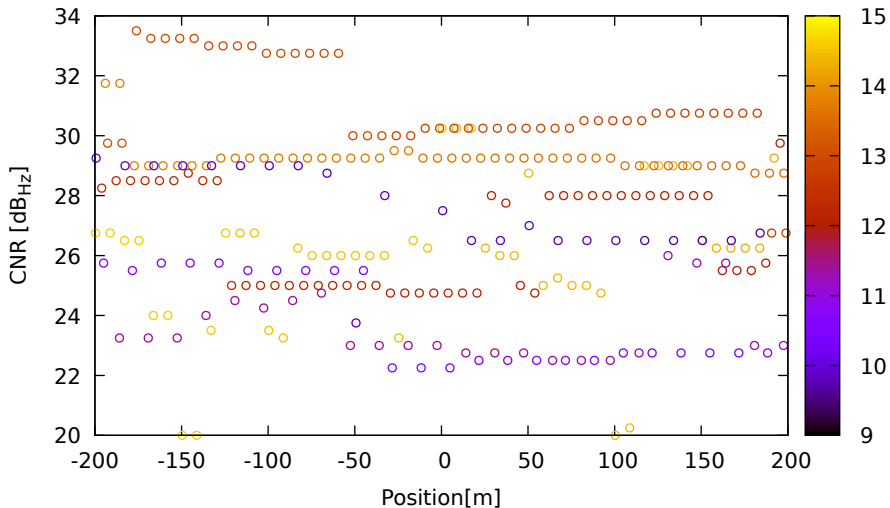
CNR vs position for C11 (B1) on Xiaomi11T - DOY 262 jam. 2
