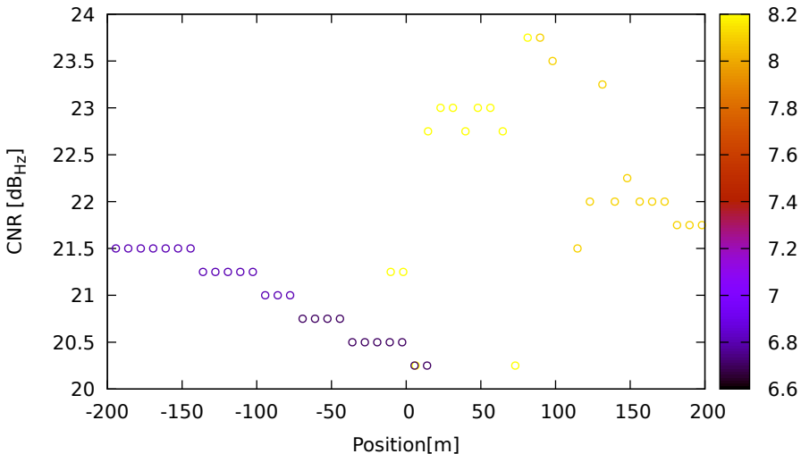
CNR vs position for C11 (B1) on Xiaomi11T - DOY 262 jam. 3
