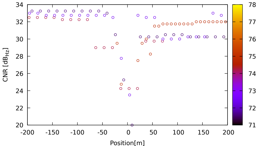
CNR vs position for C14 (B1) on Xiaomi11T - DOY 262 jam. 1
