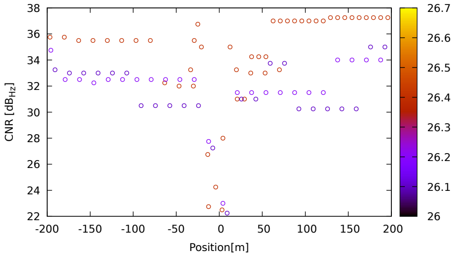
CNR vs position for C16 (B1) on Xiaomi11T - DOY 262 jam. 1
