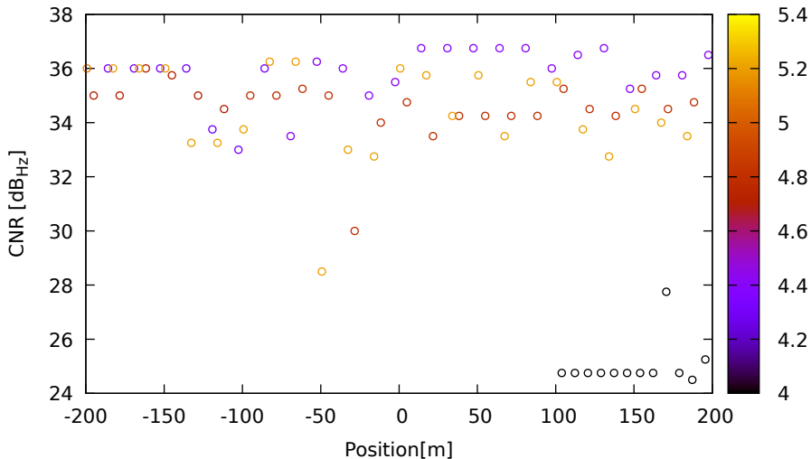
CNR vs position for C26 (B1) on Xiaomi11T - DOY 262 jam. 2
