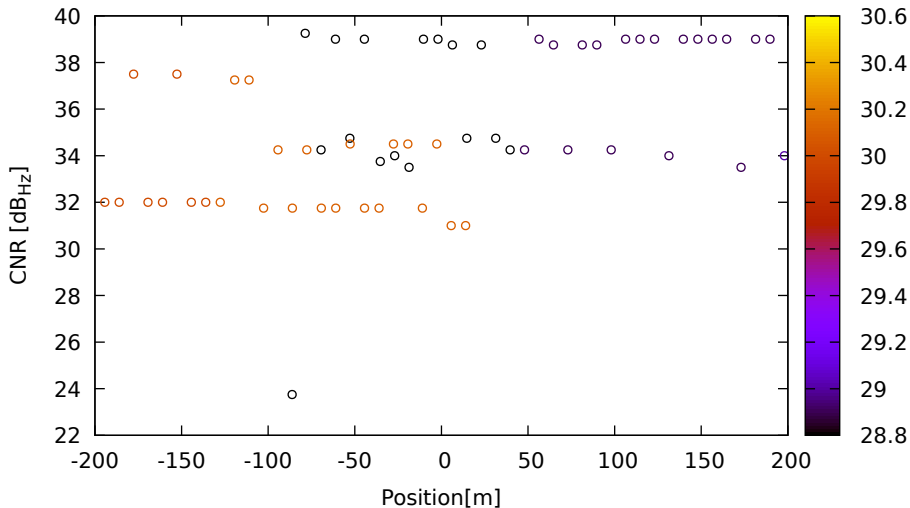
CNR vs position for C27 (B1) on Xiaomi11T - DOY 262 jam. 3
