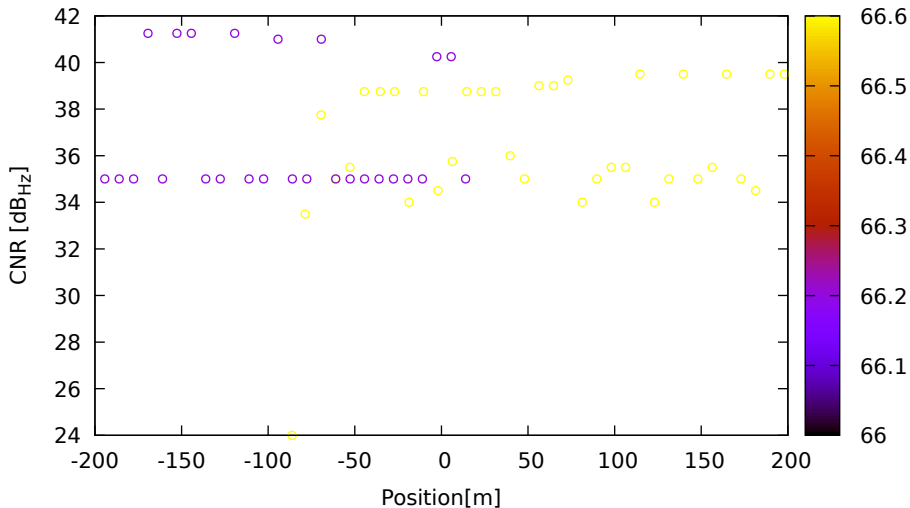
CNR vs position for C28 (B1) on Xiaomi11T - DOY 262 jam. 3
