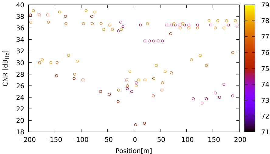
CNR vs position for C33 (B1) on Xiaomi11T - DOY 262 jam. 1
