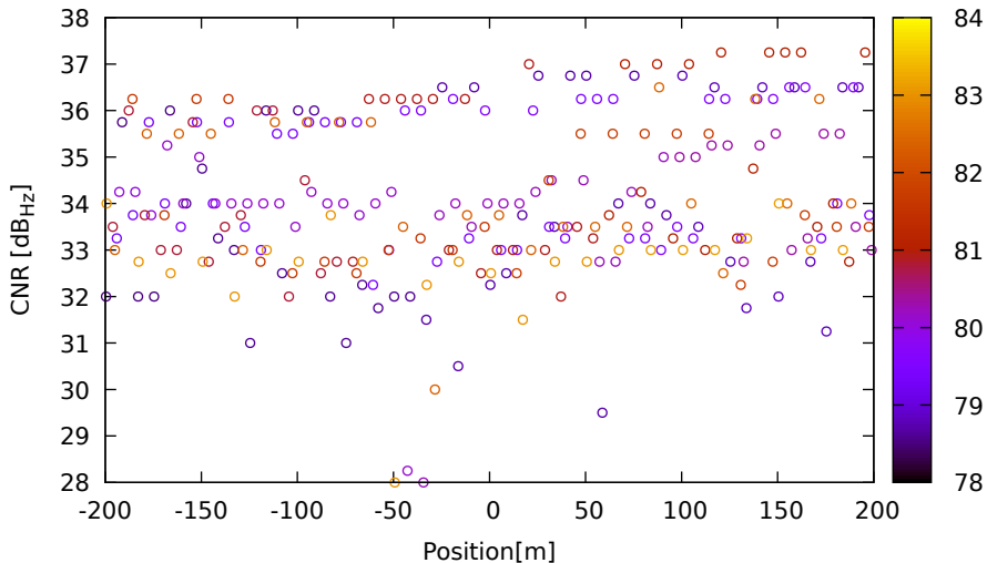
CNR vs position for C33 (B1) on Xiaomi11T - DOY 262 jam. 2
