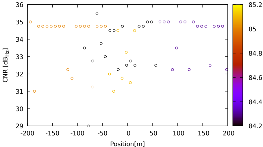
CNR vs position for C33 (B1) on Xiaomi11T - DOY 262 jam. 3
