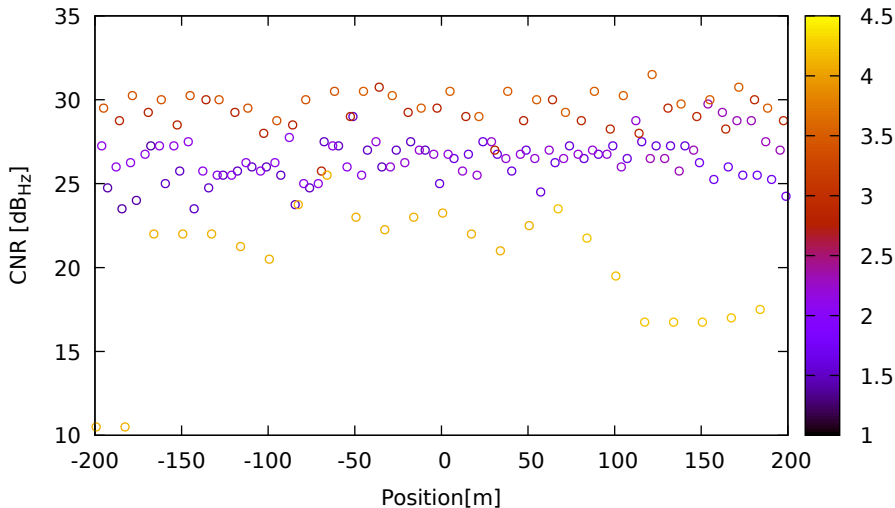
CNR vs position for E03 (E5a) on Xiaomi11T - DOY 262 jam. 2
