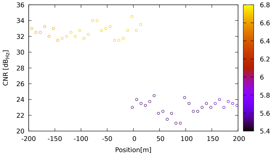
CNR vs position for E03 (E5a) on Xiaomi11T - DOY 262 jam. 3
