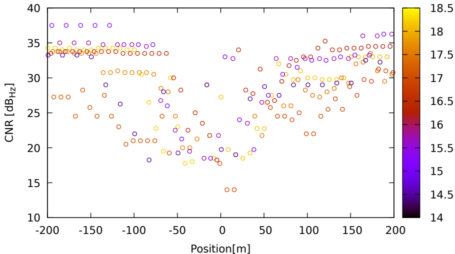
CNR vs position for E04 (E1) on Xiaomi11T - DOY 262 jam. 2
