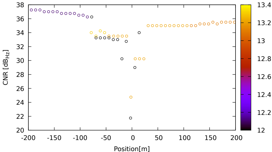
CNR vs position for E04 (E1) on Xiaomi11T - DOY 262 jam. 3
