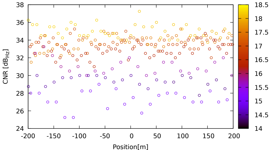
CNR vs position for E04 (E5a) on Xiaomi11T - DOY 262 jam. 2
