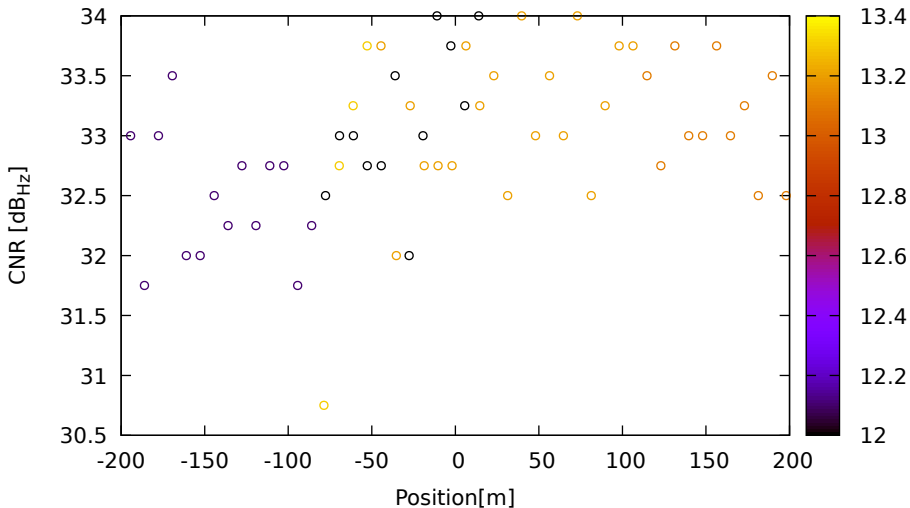
CNR vs position for E04 (E5a) on Xiaomi11T - DOY 262 jam. 3
