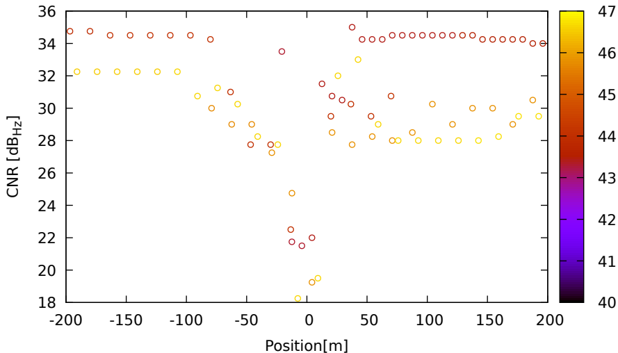
CNR vs position for E05 (E1) on Xiaomi11T - DOY 262 jam. 1
