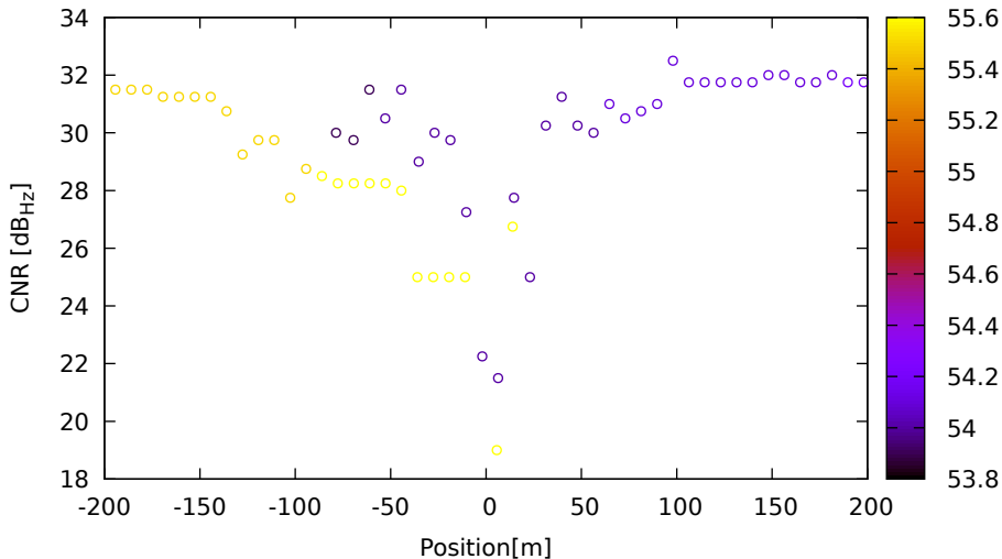
CNR vs position for E05 (E1) on Xiaomi11T - DOY 262 jam. 3
