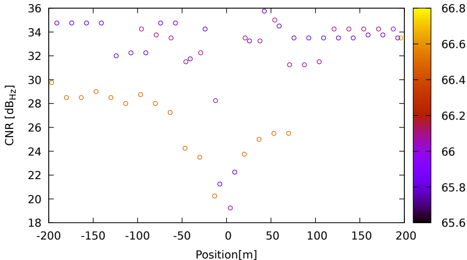
CNR vs position for E09 (E1) on Xiaomi11T - DOY 262 jam. 1
