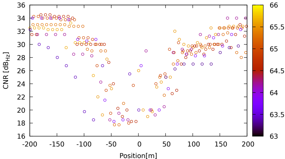
CNR vs position for E09 (E1) on Xiaomi11T - DOY 262 jam. 2
