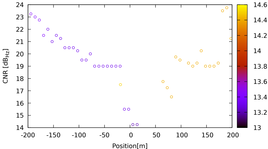
CNR vs position for E11 (E1) on Xiaomi11T - DOY 262 jam. 3
