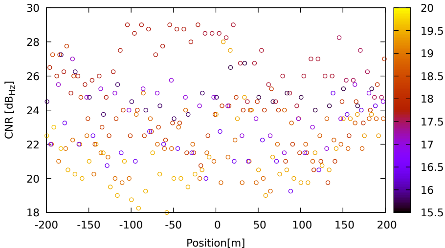
CNR vs position for E11 (E5a) on Xiaomi11T - DOY 262 jam. 2
