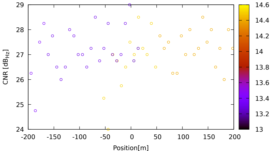
CNR vs position for E11 (E5a) on Xiaomi11T - DOY 262 jam. 3
