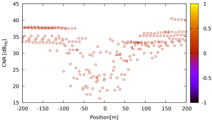
CNR vs position for E14 (E1) on Xiaomi11T - DOY 262 jam. 2
