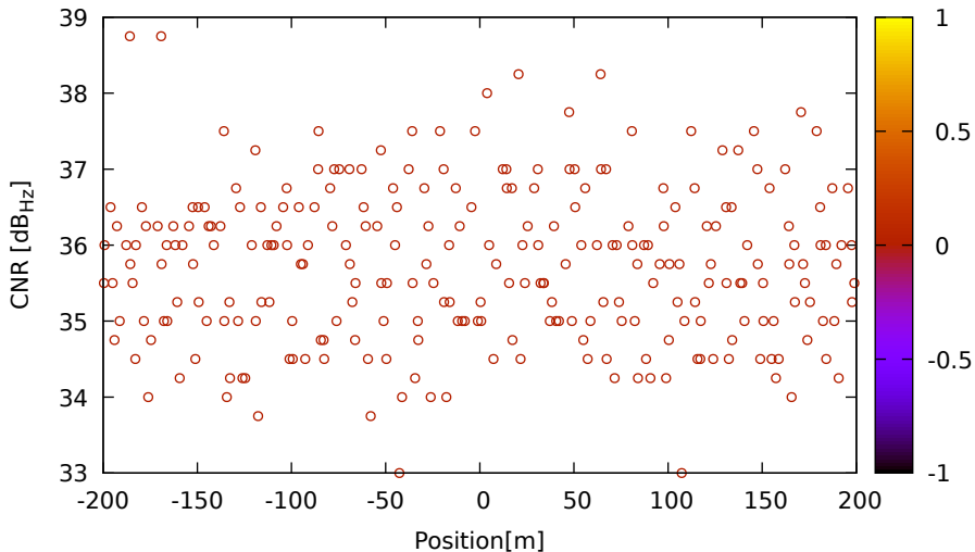
CNR vs position for E14 (E5a) on Xiaomi11T - DOY 262 jam. 2
