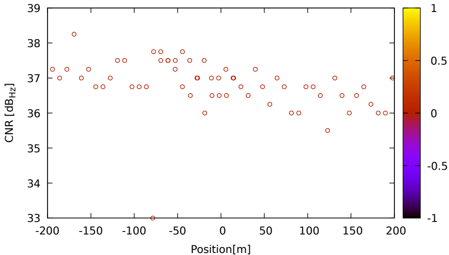
CNR vs position for E14 (E5a) on Xiaomi11T - DOY 262 jam. 3
