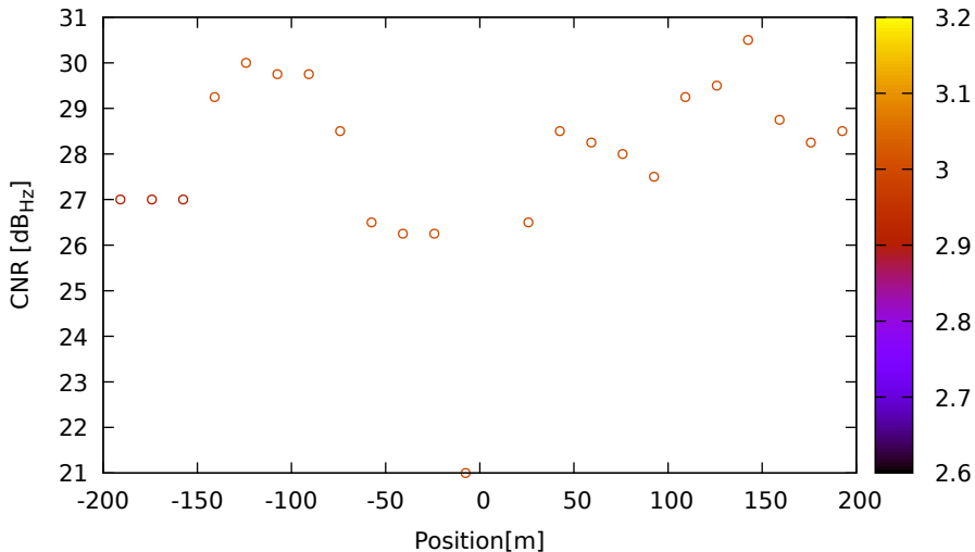
CNR vs position for E15 (E1) on Xiaomi11T - DOY 262 jam. 1
