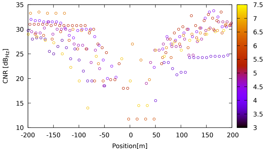
CNR vs position for E15 (E1) on Xiaomi11T - DOY 262 jam. 2
