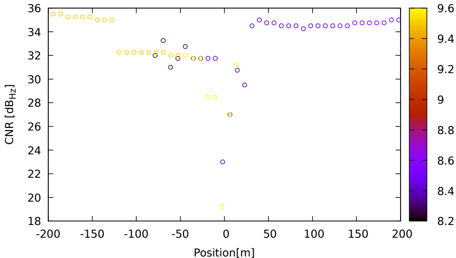
CNR vs position for E15 (E1) on Xiaomi11T - DOY 262 jam. 3
