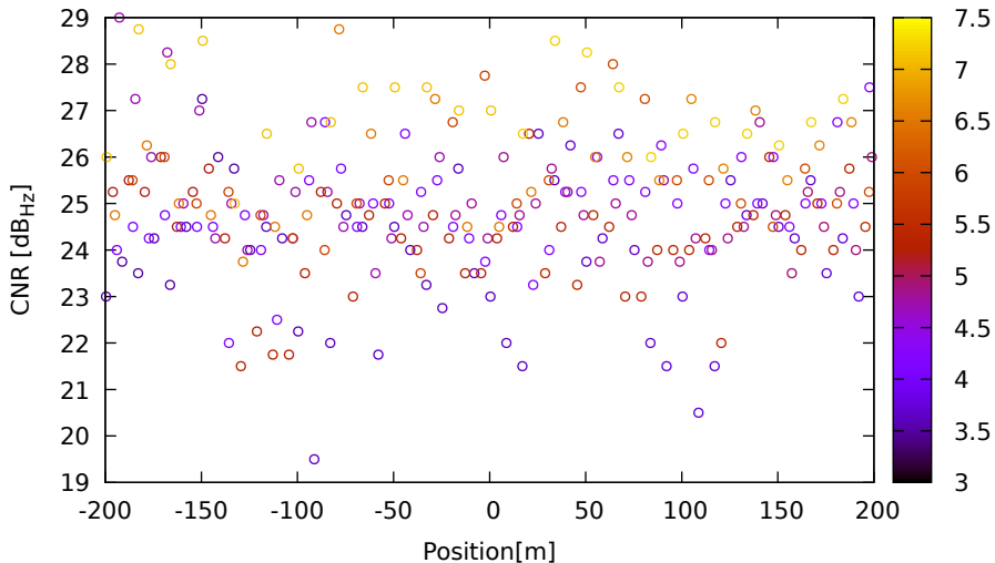
CNR vs position for E15 (E5a) on Xiaomi11T - DOY 262 jam. 2
