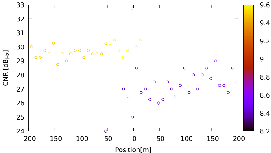
CNR vs position for E15 (E5a) on Xiaomi11T - DOY 262 jam. 3
