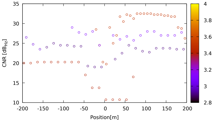
CNR vs position for E27 (E1) on Xiaomi11T - DOY 262 jam. 1
