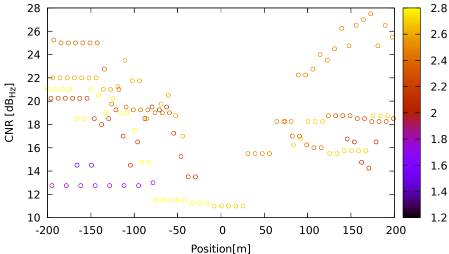
CNR vs position for E27 (E1) on Xiaomi11T - DOY 262 jam. 2
