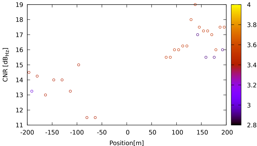
CNR vs position for E27 (E5a) on Xiaomi11T - DOY 262 jam. 1
